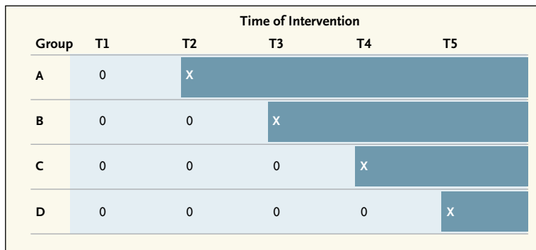
Figure 2. Stepped-Wedge Study Design Schematic.
